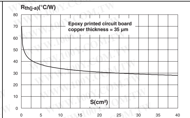
Figure 13. Thermal resistance junction to ambient versus D 2 PAK copper surface area under tab
