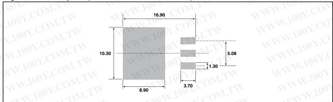
Figure 15. Footprint (dimensions in millimeters)
