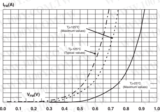
Figure 9: Forward voltage drop versus forward current (per diode, low level)
