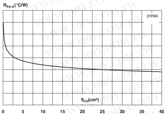
Figure 11: Thermal resistance junction to ambient versus copper surface under tab (epoxy printed board FR4, Cu = 35µm) (D 2 PAK)
