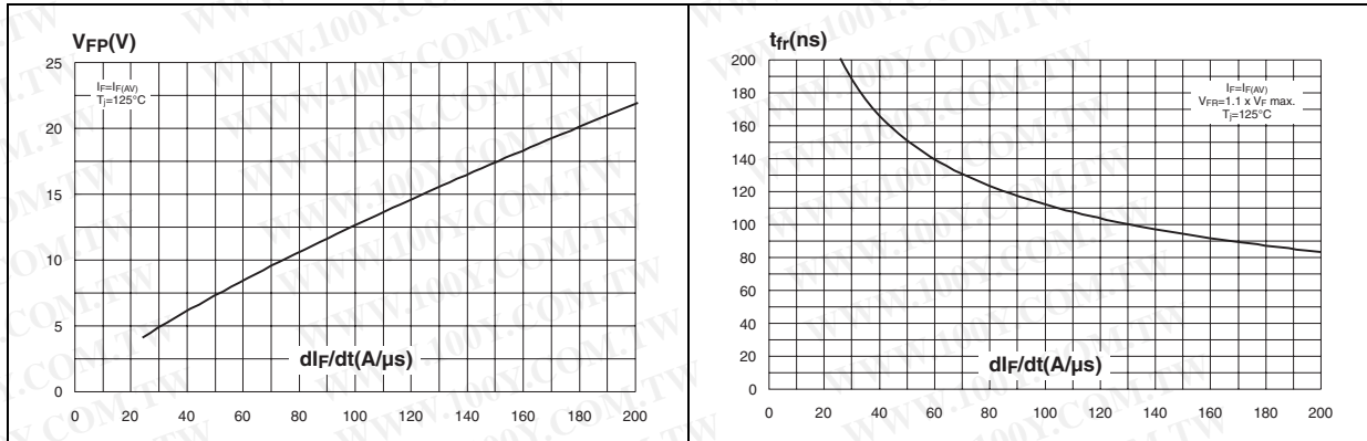
Figure 11. Transient peak forward voltage vs di_F/dt (typical values) Figure 12. Forward recovery time vs di_F/dt (typical values)
