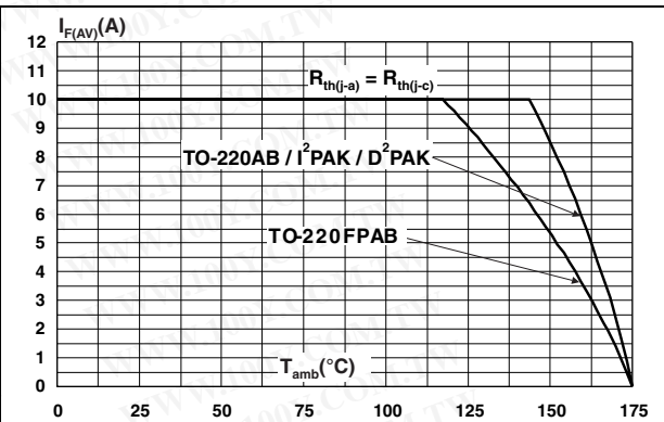
Figure 12. Average forward current versus ambient temperature (δ = 0.5, per diode)
