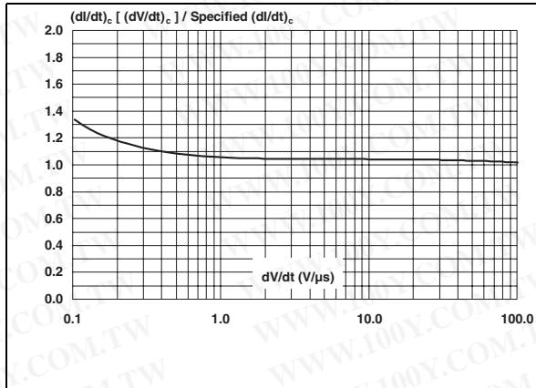
Figure 9. Relative variation of critical rate of decrease of main current (di/dt)_c versus reapplied (dV/dt)_c
