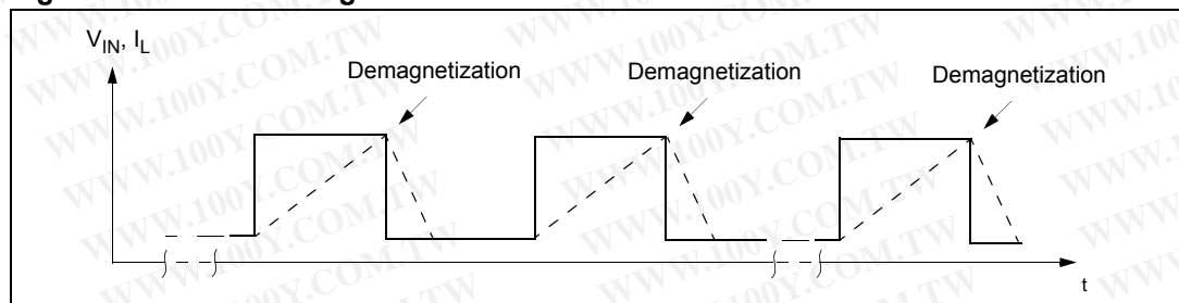
Figure 33. DPAK demagnetization
