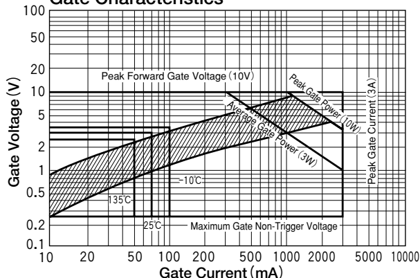
Gate Characteristics
