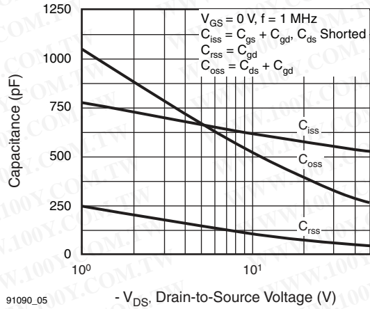
91090_05 - Fig. 5 - Typical Capacitance vs. Drain-to-Source Voltage
