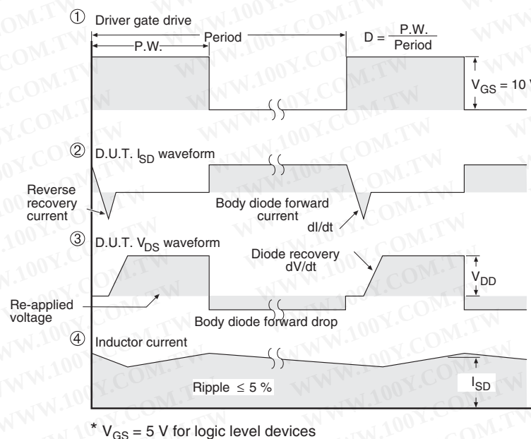
Fig. 14 - For N-Channel
