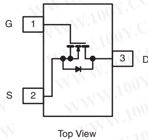
SC-70 (3-LEADS)
