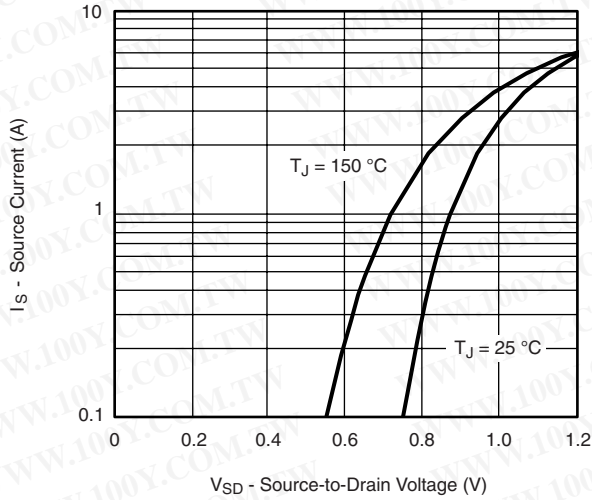
Forward Diode Voltage
