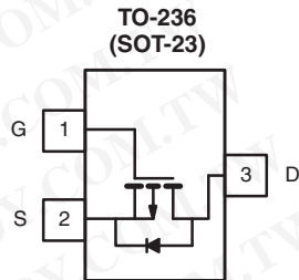
Si2301CDS (N1)* * Marking Code
