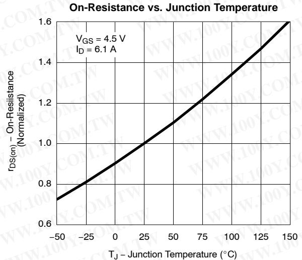
FIGURE 4. Si3434DV
