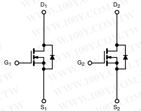
N-Channel MOSFET
