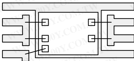
a) 8-Pin Single-Pad TSSOP
