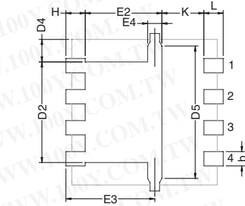
Backside View of Single Pad
