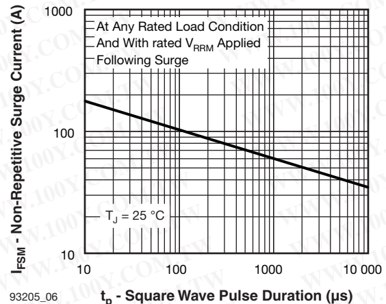
93205_06 t p - Square Wave Pulse Duration (μs) Fig. 6 - Maximum Non-Repetitive Surge Current
