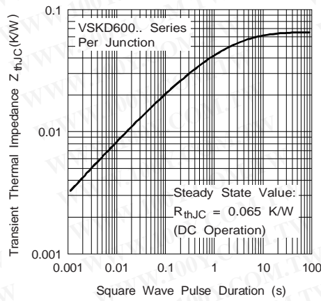
Fig. 10 - Thermal Impedance Z θJC Characteristic
