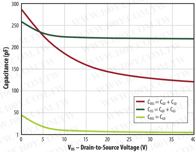
Figure 5a: Capacitance
