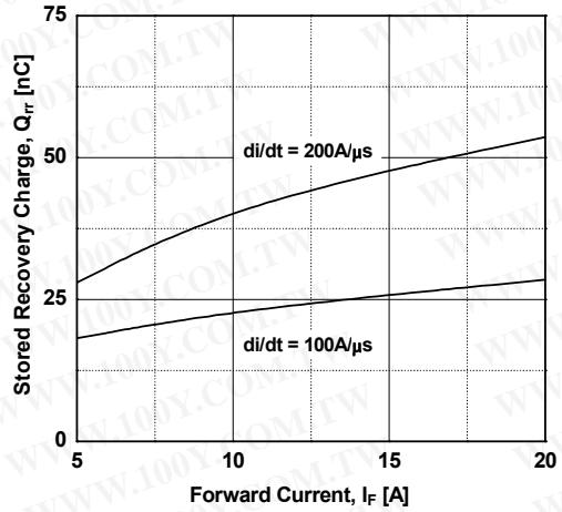
Figure 24. Stored Charge
