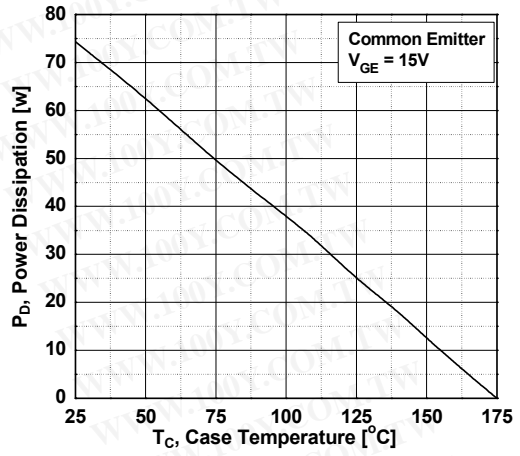
Figure 20. Power Dissipation
