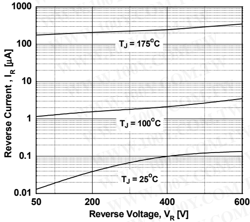
Figure 23. Reverse Current
