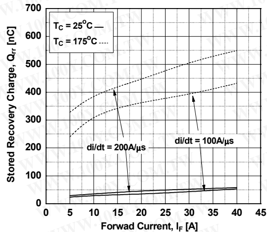
Figure 24. Stored Charge
