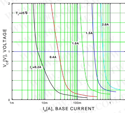
Figure 5. Typical Collector Saturation Voltage
