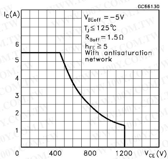
Reverse Biased SOA
