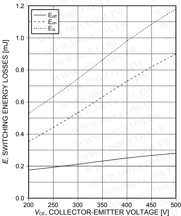
Figure 15. Typical switching energy losses as a function of collector emitter voltage (inductive load, T_{vj}=150^{\circ}\text{C} , V_{GE}=15/0\text{V} , I_C=25\text{A} , r_G=12\Omega , Dynamic test circuit in Figure E)
