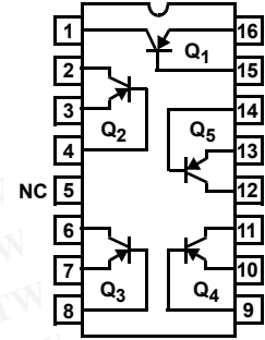
HFA3128 TOP VIEW
