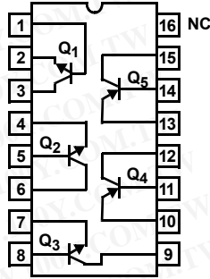
HFA3096 TOP VIEW
