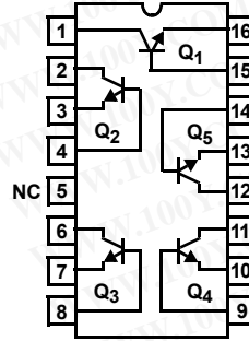
HFA3127 TOP VIEW
