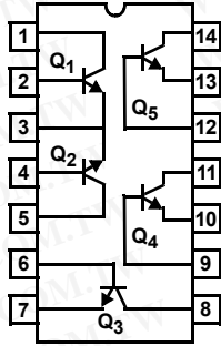
HFA3046 TOP VIEW
