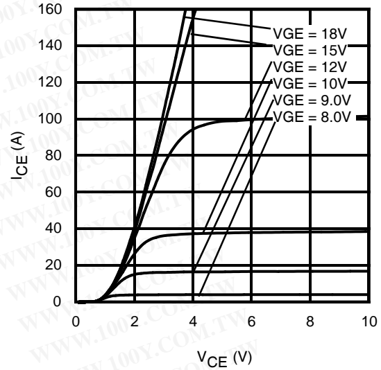
Fig. 7 - Typ. IGBT Output Characteristics T_J = 25^\circ C; t_p = 20\mu s
