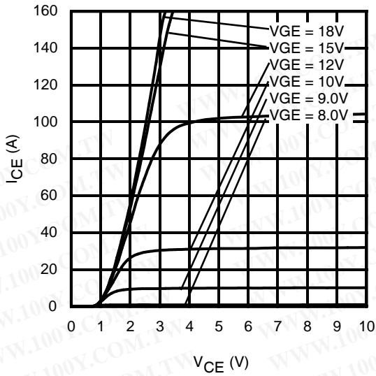
Fig. 6 - Typ. IGBT Output Characteristics T_J = -40^\circ C; t_p = 20\mu s
