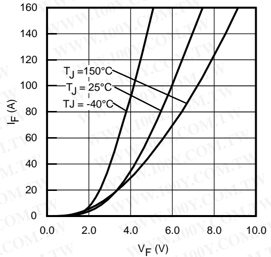
Fig. 9 - Typ. Diode Forward Characteristics t_p = 20\mu s
