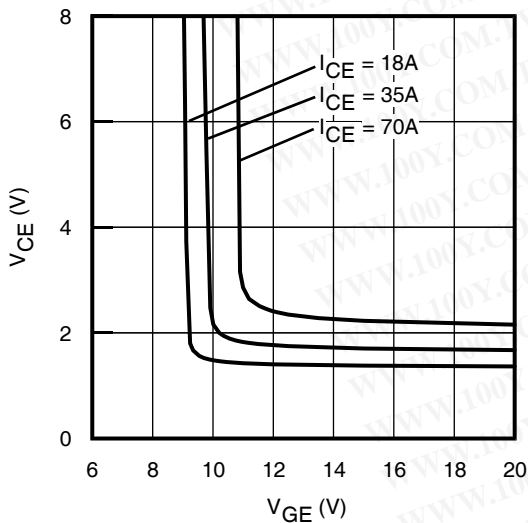
Fig. 10 - Typical V_{CE} vs. V_{GE} T_J = -40^\circ C
