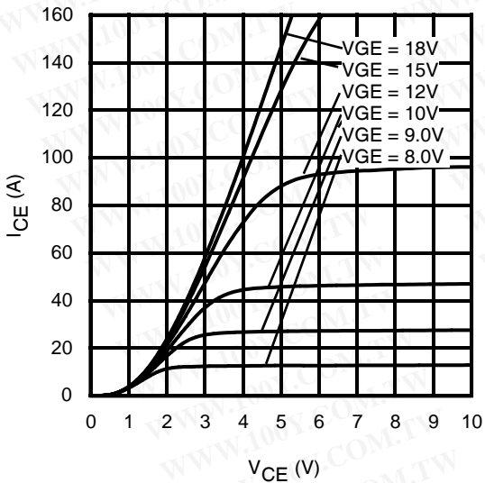
Fig. 8 - Typ. IGBT Output Characteristics T_J = 150^\circ C; t_p = 20\mu s
