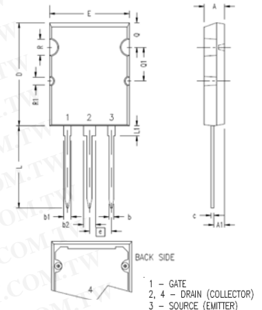
PLUS264™ (IXFB) Outline
