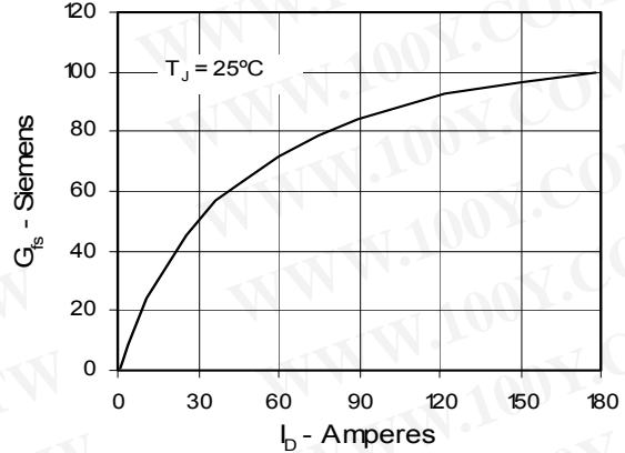
Fig. 8. Transconductance
