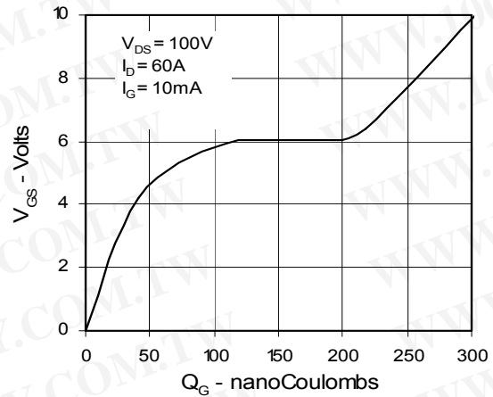
Fig. 10. Gate Charge
