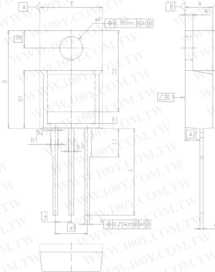
PG-TO-220-3-1, PG-TO220-3-21
