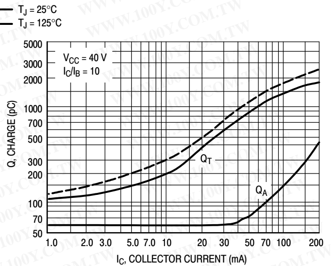
Figure 4. Charge Data
