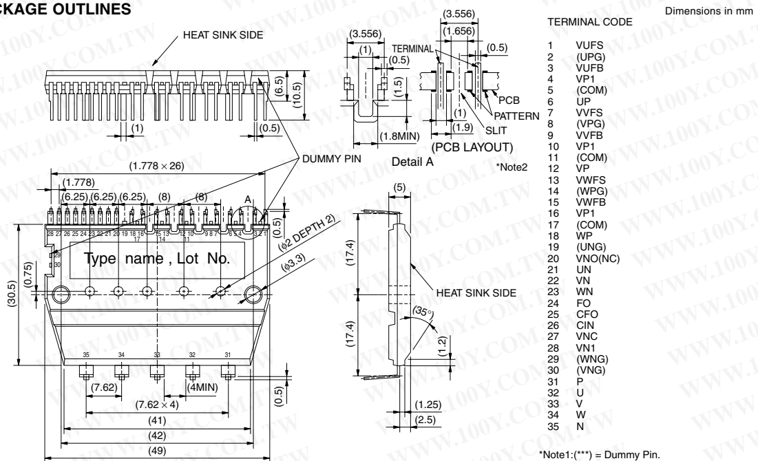
Fig. 1 PACKAGE OUTLINES
