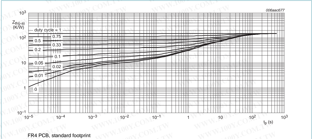
Fig 4. Transient thermal impedance from junction to ambient as a function of pulse duration for SOT223; typical values
