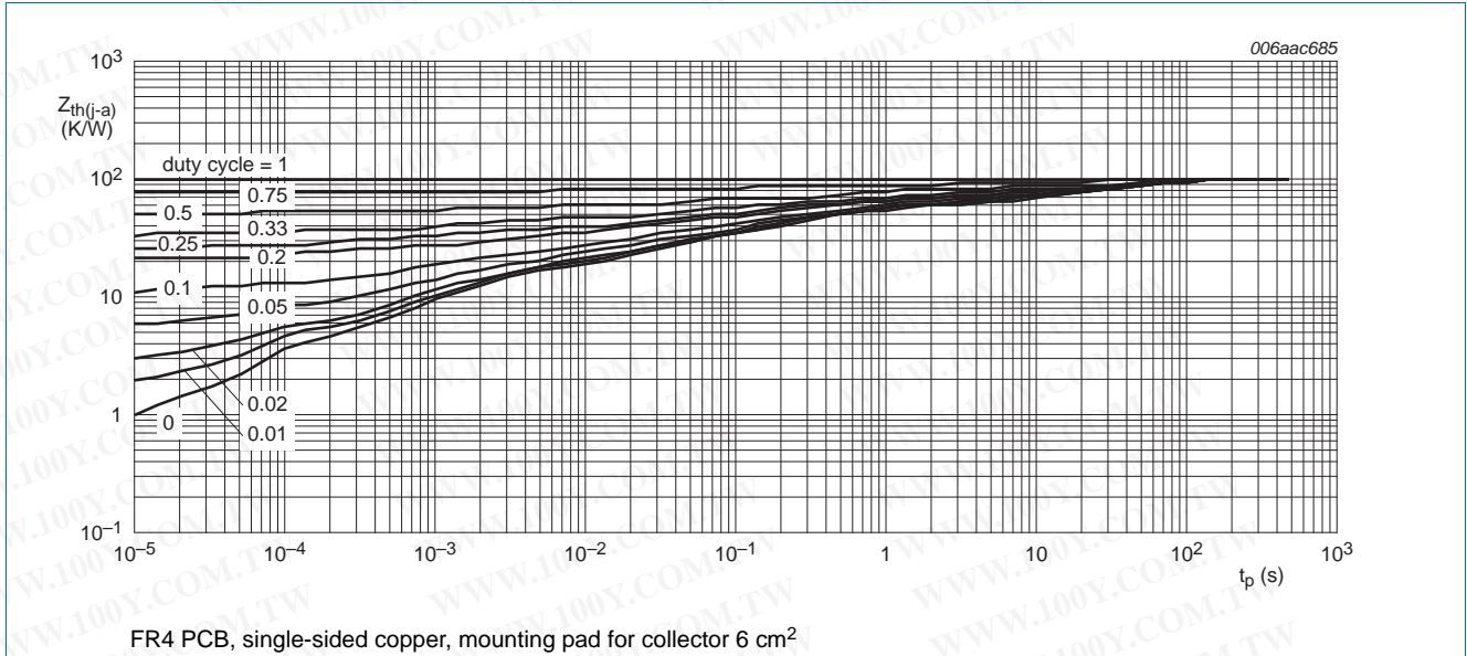
Fig 12. Transient thermal impedance from junction to ambient as a function of pulse duration for SOT1061; typical values
