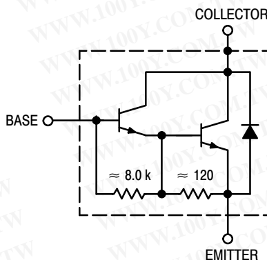
Figure 13. Darlington Schematic
