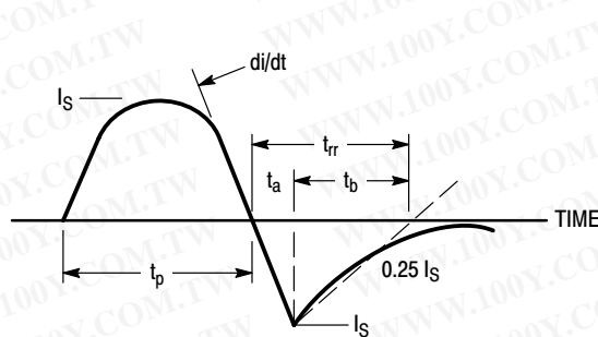
Figure 14. Diode Reverse Recovery Waveform
