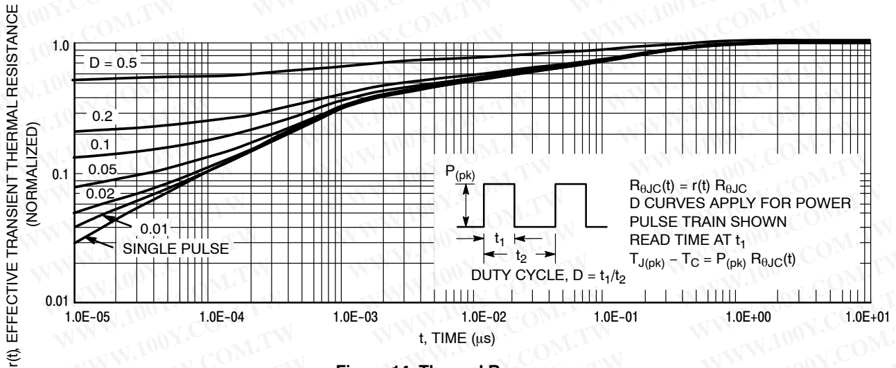
Figure 14. Thermal Response
