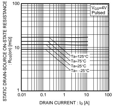
Fig.5 Static Drain-Source On-State Resistance vs. Drain Current(IV)
