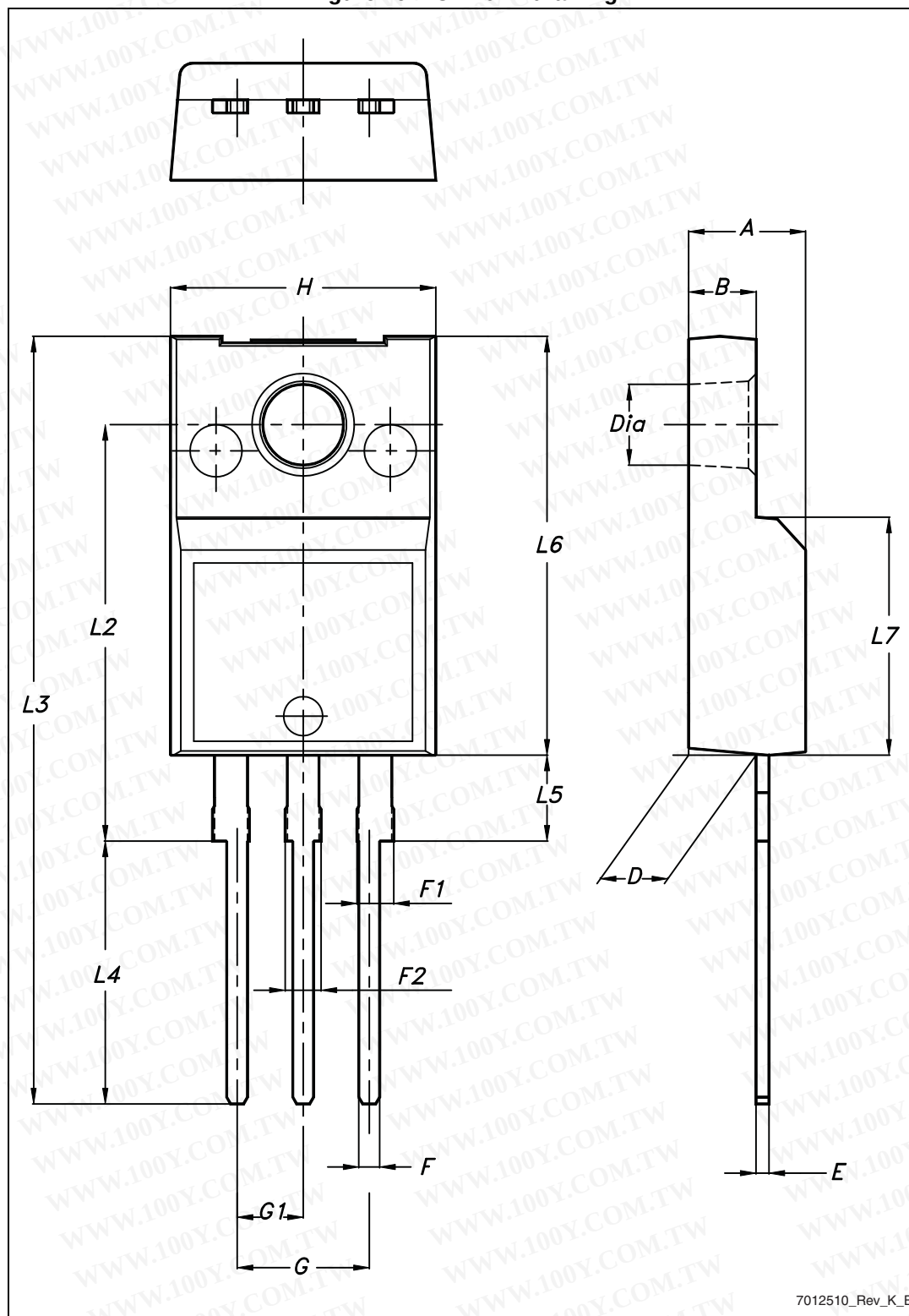
Figure 29. TO-220FP drawing
