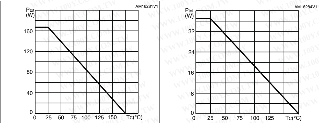
Figure 10. Power dissipation vs. case temperature for D²PAK and TO-220 Figure 11. Power dissipation vs. case temperature for TO-220FP
