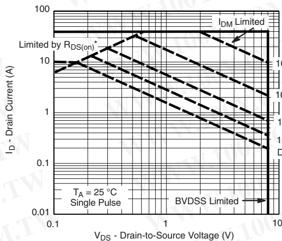
Safe Operatin Area
