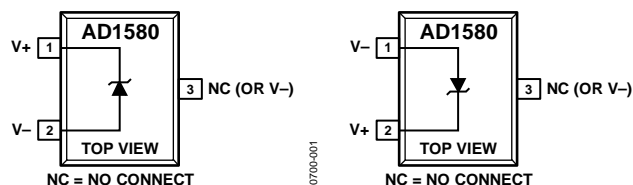
Figure 1. SOT-23
