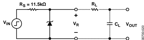
Figure 20. Turn-On, Settling, and Transient Test Circuit
