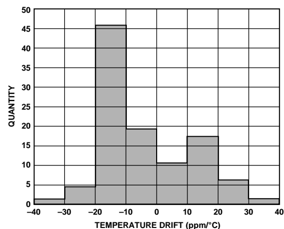
Figure 3. Reverse Voltage Temperature Drift Distribution
