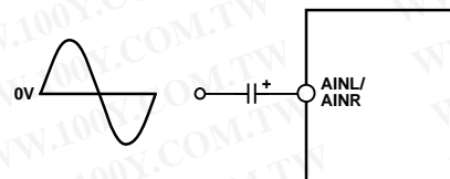
Figure 44. AC-Coupled Input Signal
