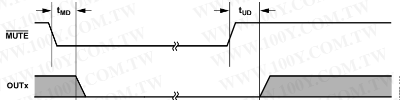
Figure 2. Mute and Unmute Delay Timing
