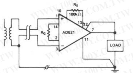
a). Transformer Coupled, Direct Return
