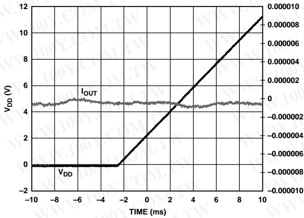
Figure 43. Output Current vs. Time on Power-Up
