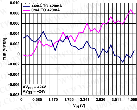
Figure 28. Total Unadjusted Error vs. V_{IN} , External R_{SET} Resistor
