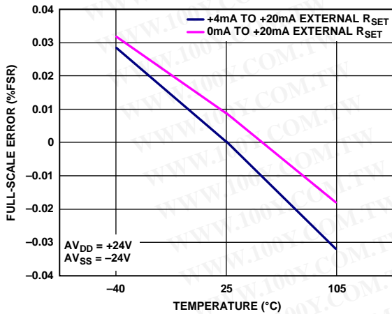
Figure 38. Full-Scale Error vs. Temperature, External RSET Sense Resistor
