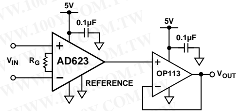
Figure 52. Output Buffering
