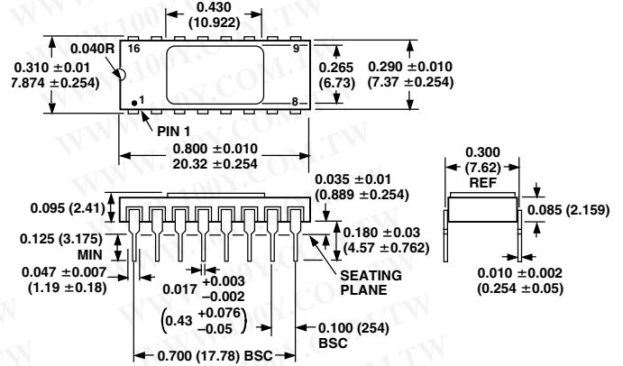
16-Lead Ceramic DIP (D-16)
