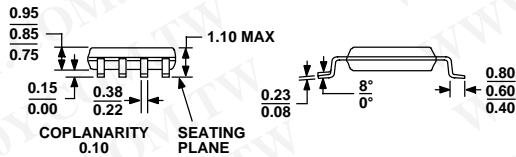
Figure 36. 8-Lead Mini Small Outline Package [MSOP] (RM-8) Dimensions shown in millimeters
