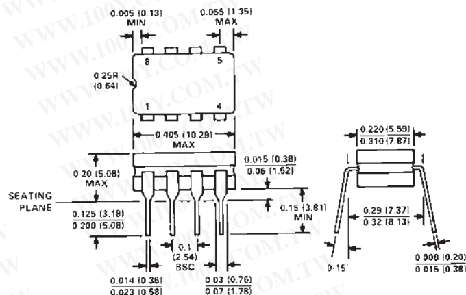
8-Pin Cerdip (Q-8) Package
