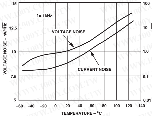
Figure 9. Voltage and Current Noise Spectral Density vs. Temperature
