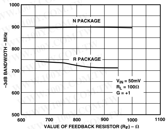
TPC 16. -3 dB Bandwidth vs. R_F , G = +1
