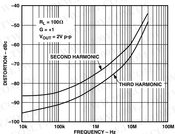
TPC 17. Distortion vs. Frequency, R_L = 100\Omega
