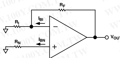
Figure 5. Output Offset Voltage
