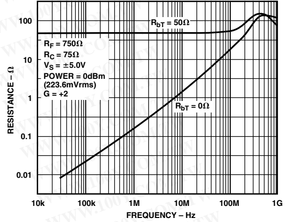
TPC 28. Output Resistance vs. Frequency
