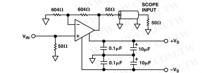
Figure 3. Test Circuit; Gain = -2
