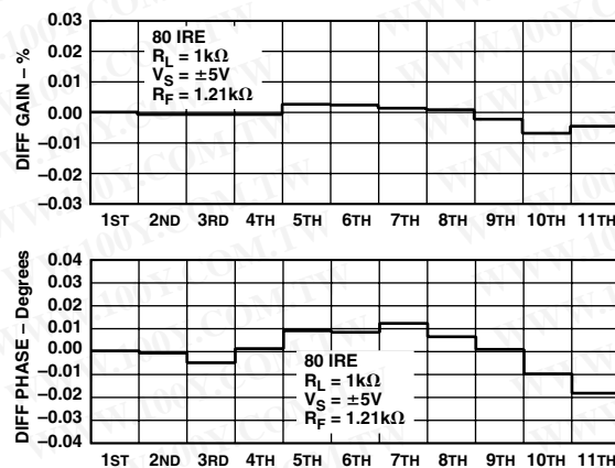
TPC 24. Differential Gain/Phase, R_L = 1k\Omega
