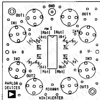
NONINVERTER DIP
